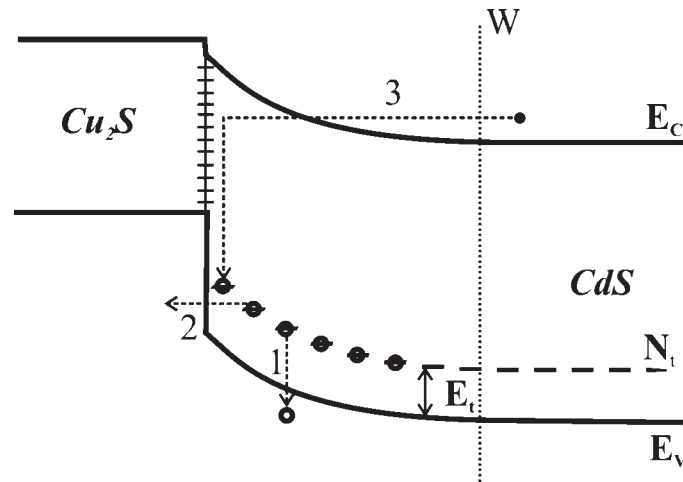
Fig. 1. CdS-Cu 2 S heterojunction band diagram showing the possible ways of nonequilibrium charge removal from SCR.
