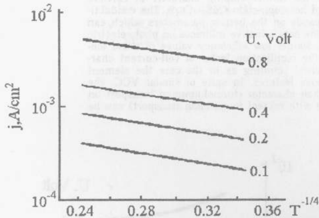
Fig. 3. Temperature dependences of direct current for CdS—Cu 2 S heterojunction in Mott coordinates:
